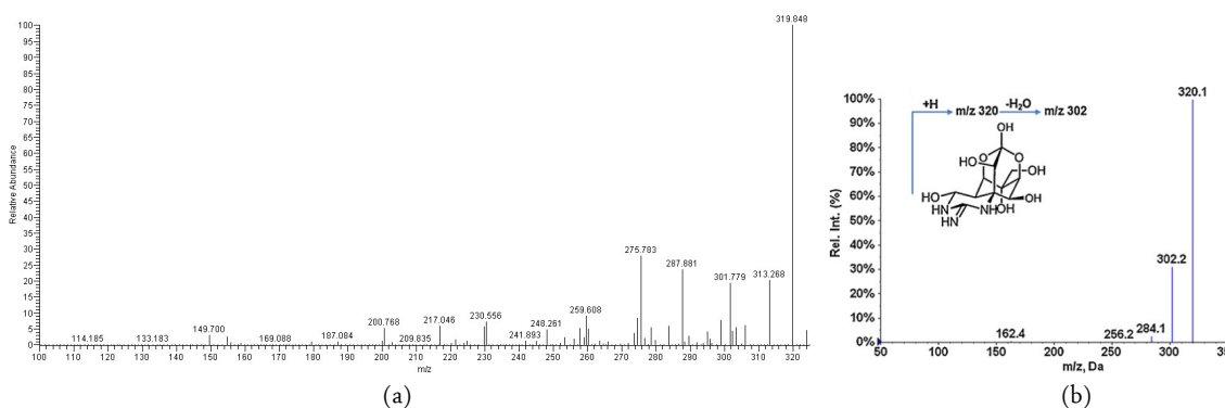
Figure 2. Product ion mass spectra of with LC-MS/MS of T. fluviatilis liver extract (A); Authentic TTX (B) [16]. Predominant peaks showed at m/z 320, in accordance to TTX molecular weight, 302 m/z and 257 m/z for TTX-related substances. Other peaks indicating presence of other non TTX-related substances.
