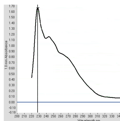
Figure 1. Spectrums of UV absorption of alkaline hydrolyzates of TTX fraction from T. fluviatilis liver extract and authentic TTX with UV spectroscopy nanodrop is around 240 nm
